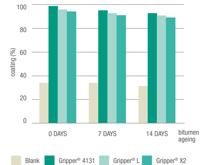
BOILT TEST Granite, 50%70 straight asphalt, 0,3% Grippeer®, 10' boil, 0,05 g/L Na 2 CO 3
